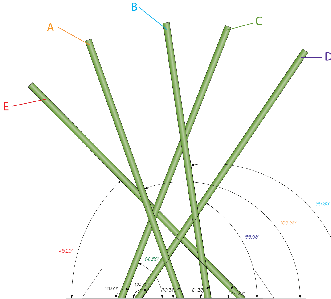
SIDE A ANGLE OF PIPES
