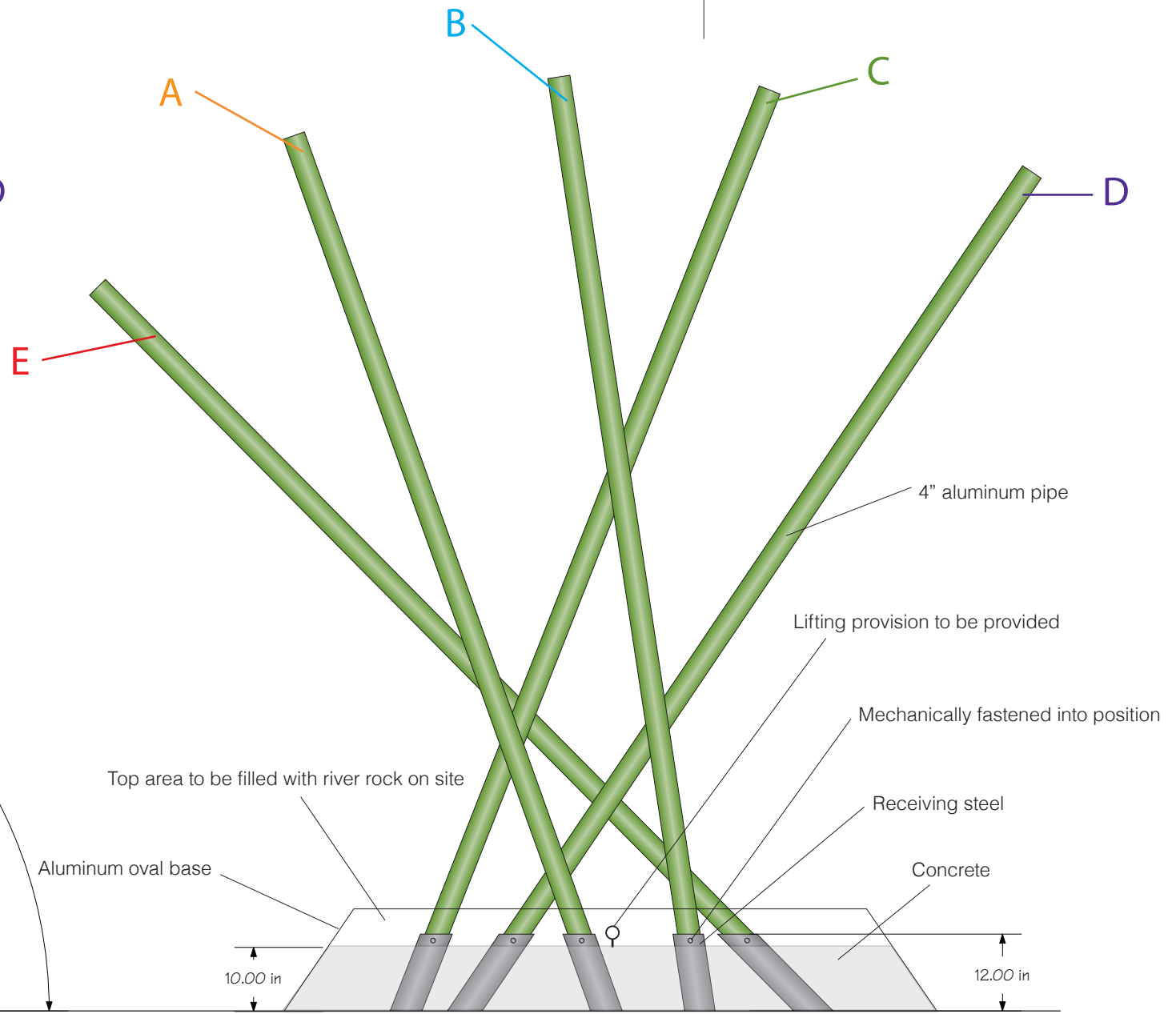
SIDE A - ILLUSTRATION OF ALUMINUM ANGLE SLEEVED INTO RECEIVING STEEL PIPES
